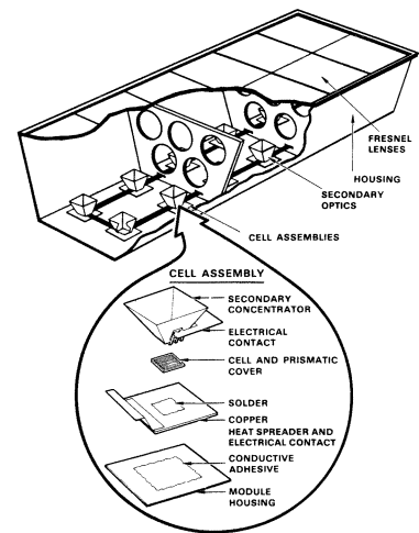
Sandia Schematic of Sandia's photovoltaic concentrator module.
