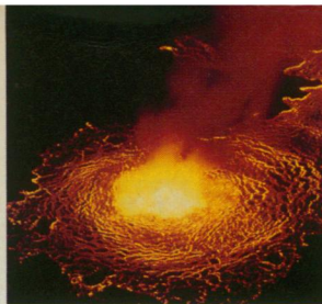
Molten lava rock continually reshapes the Earth's surface.
