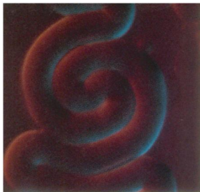
Test tube recreation of Earth's primeval chemistry.
