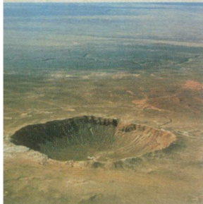
Arizona's Meteor Crater: one of Earth's many asteroid impact sites.
