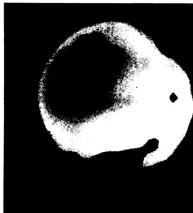
Radio emissions from Mercury's "hot poles" suggest the planet has no molten core.
