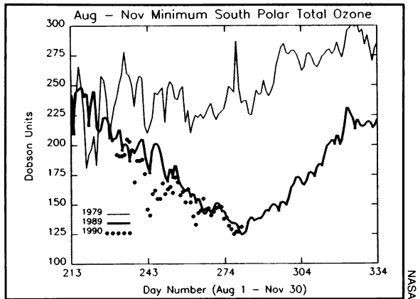
Satellite measurements of Antarctic ozone loss in 1990 and other years.
