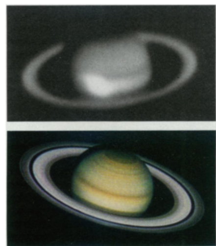
Image of Saturn (top photo), taken last week from Earth, shows extent of giant spot. Hubble's Saturn image (bottom photo), released last week but taken before the white spot's debut, can't rival Voyager's close-up photos taken a decade ago. But it has the same clarity as if Saturn were only twice the moon's distance from Earth, and viewed with the naked eye.
