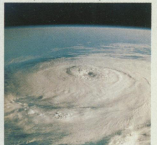
Earth's rotation helps create hurricanes, as seen from space.
