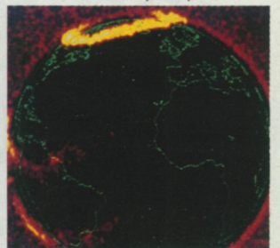
"Northern Lights"... Earth's magnetic field clashing with the solar wind.
