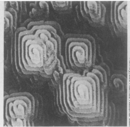
Whorls apart? These STM images, made by separate research teams in Switzerland (left) and the United States, provide remarkably similar views of the terraced surfaces of superconducting films.
