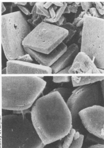
Phosphonate compounds cause rhombic barium sulfate crystals (top) to develop curved sides (bottom).
