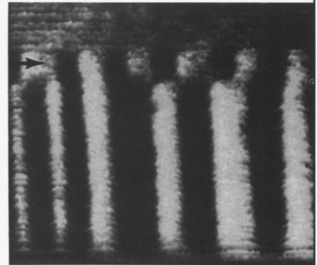
Created with magnetic-force STM, this image of a computer disk drive shows the magnetic pattern of “erased” data (arrow) as well as currently stored information.
