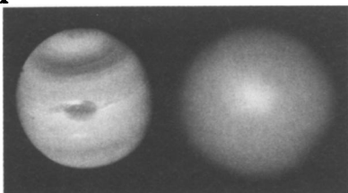
Left: Neptune image taken by Voyager 2 in 1989 shows a bright area just above the planet's Great Dark Spot. Right: Image taken from Earth shows same feature depicted as bright blob.
