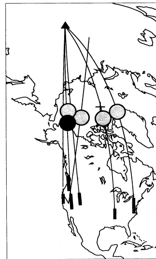
Rumblings from an underground nuclear test (black triangle) helped scientists pinpoint an anomalous region of Earth's mantle, located 2,700 km beneath the dark circle. Dark rectangles mark the seismic networks in the United States and Canada that detected the region. White circles represent homogenous mantle.
