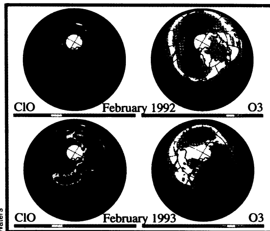
In the left column, maps of chlorine monoxide (ClO) measured by the UARS satellite show the Arctic had much more of the ozone-destroying chemical in February 1993 than in February 1992. Right figures compare average ozone concentrations from February 15 through March 6 in both years, with red and orange indicating greatest amounts. Concentrations for 1993 were lower than those for 1992.
