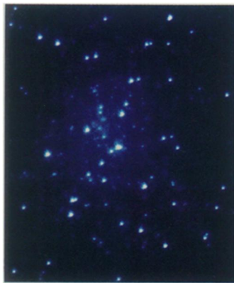
False-color image depicts a new class of stars in M15.
