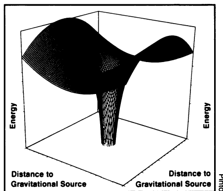
This drawing shows how the strong gravitational field of a typical neutron star affects the potential energy of an electron bound to an atom situated at the star's surface. The star's gravitational force stretches the atom in much the same way the moon induces tides on Earth. This stretching adds a waviness to the corresponding potential energy diagram.
