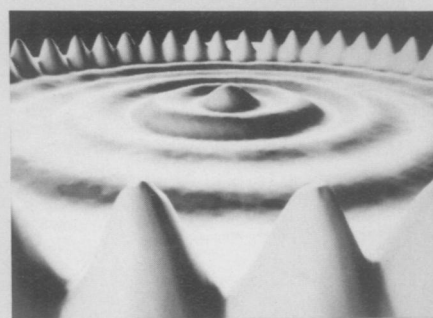
Iron atoms in a circular "corral" cause electron standing waves.
