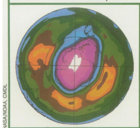
In the satellite image, from Sept. 28, magenta hues indicate ozone hole, with white marking the most depleted region. Graph shows vertical profiles of ozone over South Pole. Black line represents conditions prior to hole's development. Green, blue, and red lines show how ozone disappeared over a six-week period.
