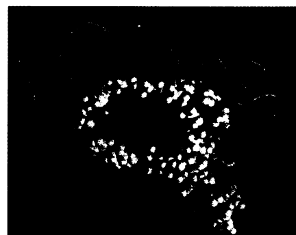
Computer graphic of DNA (balls) bound to the underside of TBP (ribbon).
