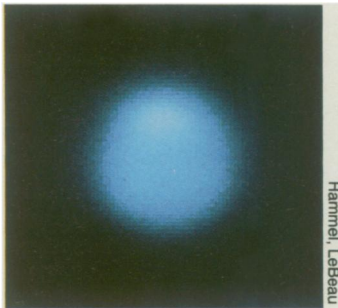
Near-infrared image of Neptune shows bright region in the planet's northern hemisphere.
