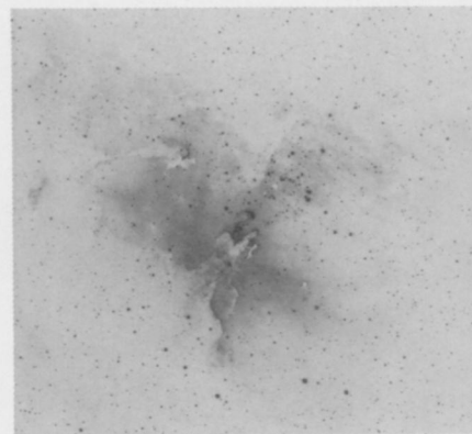
Stars in the young cluster NGC 6611, with the Eagle nebula at center.
