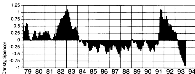
Stratospheric temperatures (in degrees Celsius) rise and then plummet after Pinatubo eruption in June 1991.
