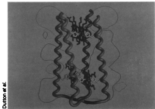
A protein maquette.
