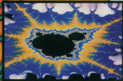
Mandelbrot fractal
