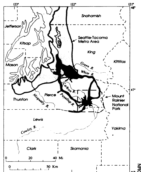
Mount Rainier has spawned large mudflows (dark shading) that swept toward Puget Sound through now heavily populated land.
