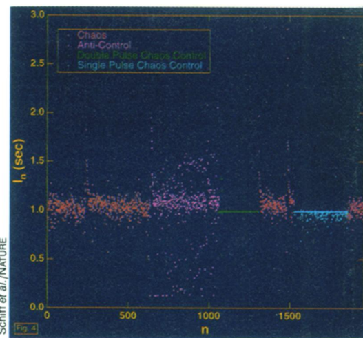
This chart shows how dispersed chaotic pulses can be made more erratic (anti-control), less erratic with single control pulses, and practically synchronized with double control pulses.
