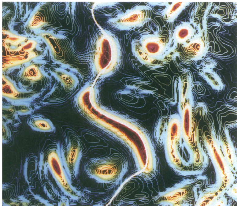
This slice through a simulated flame reveals features on the scale of a few millimeters. As a measure of turbulence, the colored blobs represent the local rotation rate of the gas (maximum values indicated in red). The white contour lines show the overall reaction rate.
