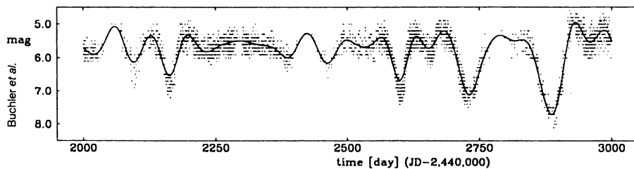
Graph shows that the star R Scuti brightens and fades erratically over time.
