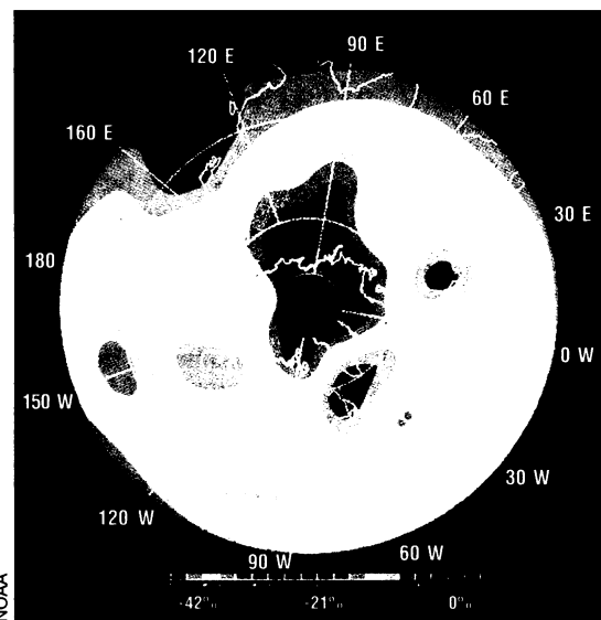
Comparison of March ozone values in 1979 and 1995. Red indicates no change. Green shows where 1995 amounts fell 20 percent below 1979 values.
