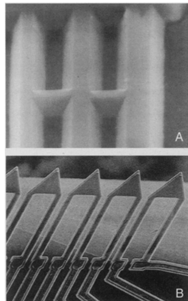
A scanning electron microscopy of silicon wires, made with an atomic force microscope (A); an array of five tips (B).
