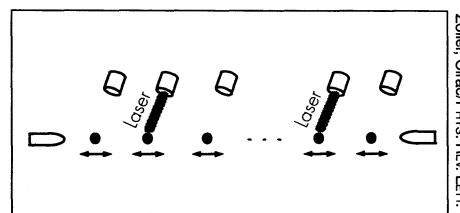
Oscillating ions in a linear trap interacting with different laser beams.
