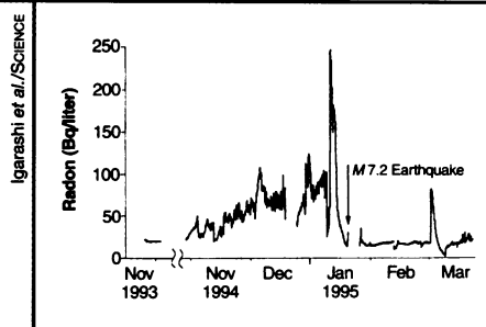
Groundwater radon peaked before Kobe quake.
