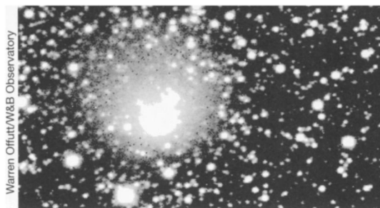
Comet Hale-Bopp imaged with a 0.6-meter telescope on July 24.
