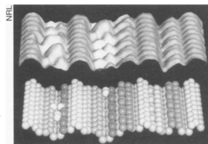
Scanning tunneling microscope image (top) and computed atomic reconstruction (bottom) showing atomic structure of a newly characterized silicon surface.
