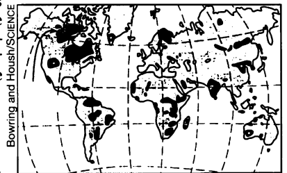
Black denotes rock older than 2.5 billion years. Star shows world's oldest rocks.
