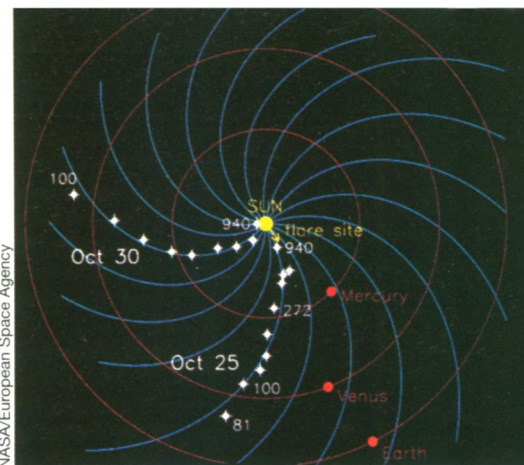
Map reveals spiral shape of the sun's interplanetary magnetic field.
