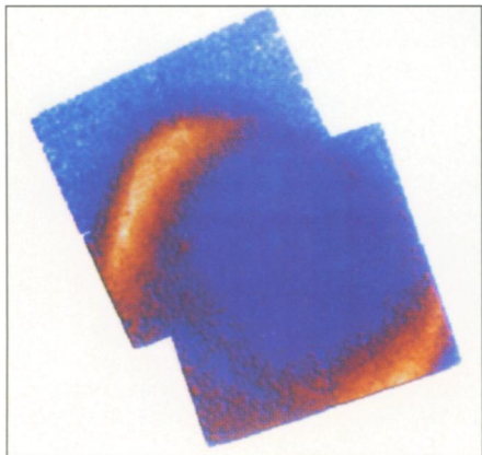
Koyama, E. V. Gotthelf, et al./NATURE
