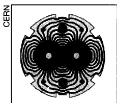
Representation of the magnetic field that confines and bends a pair of proton beams inside a superconducting magnet at the Large Hadron Collider.
