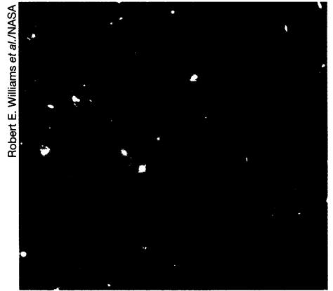
Section of the Hubble Deep Field.
