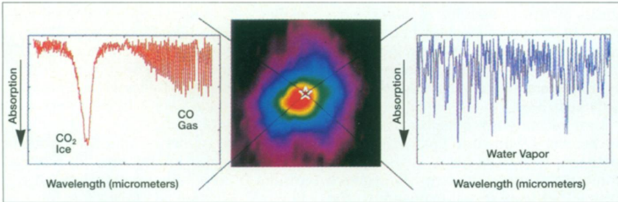
Center: Radio image shows the densest part of the molecular cloud that gave birth to the young, massive star GL 2591 (denoted by star). Left: ISO absorption spectrum shows frozen carbon dioxide (CO 2 ) and gaseous carbon monoxide (CO). Right: ISO spectrum reveals abundant water vapor in the direction of GL 2591.
