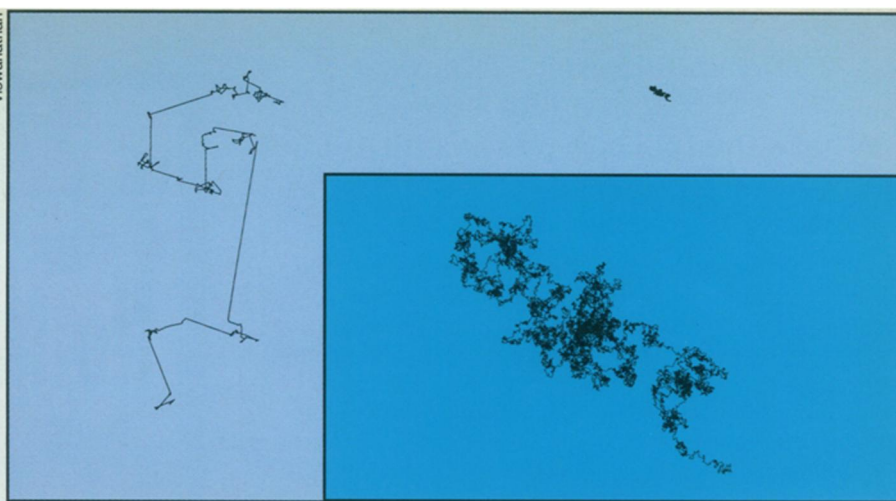
A comparison of a Lévy flight (left) to a Brownian random walk (top right) for the same number of steps reveals that a Lévy flight covers a considerably larger area. An enlargement of the Brownian random walk (inset) shows that this type of random motion lacks the long segments of a Lévy flight.
