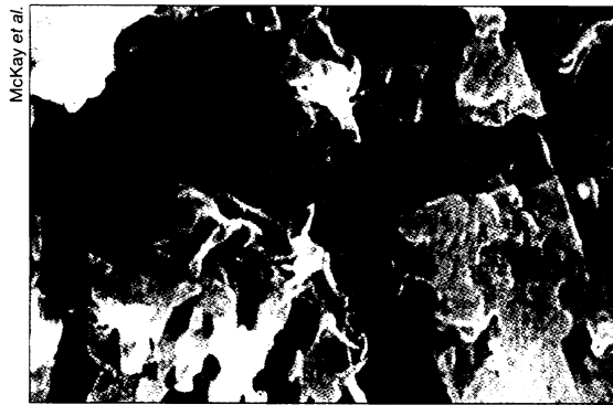
Colorized photo of acid-etched fragment of ALH84001 shows a coating that could be a biofilm.
