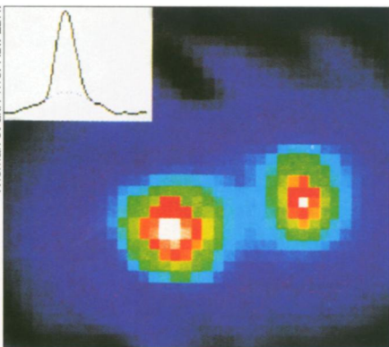
This false-color image shows two atomic clouds representing the different quantum states created simultaneously during the cooling of rubidium atoms to temperatures below 250 microkelvins. Inset: Cross section of cloud on left shows concentration of coherent atoms.
