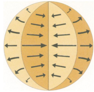
Model of the gas oscillations that may occur across sectors of the surface of 51 Pegasi. Near the edge of the star, such motions could be observed from Earth and interpreted as a wobble.
