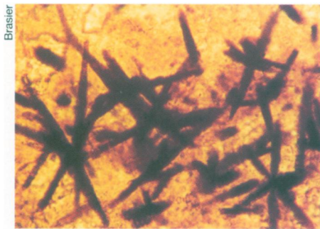
Pieces of the oldest known sponges.
