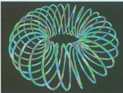
Example of a complex torus knot.
