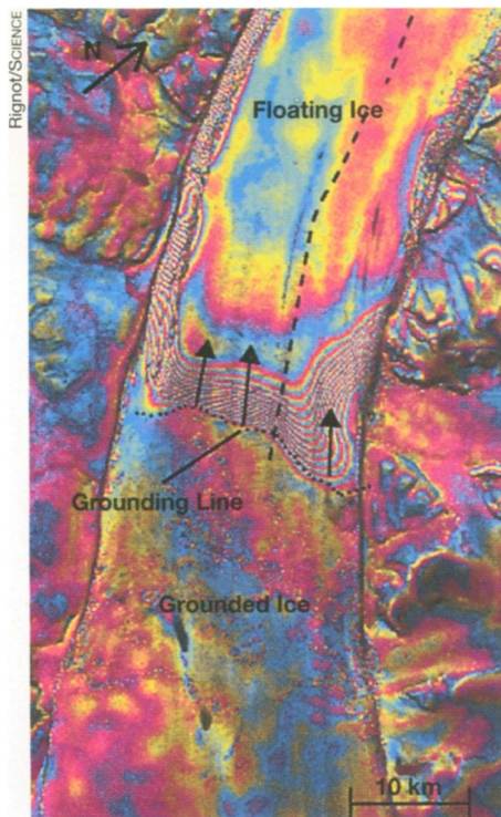
Radar image of northern Greenland glacier. Arrows show direction of ice flow.
