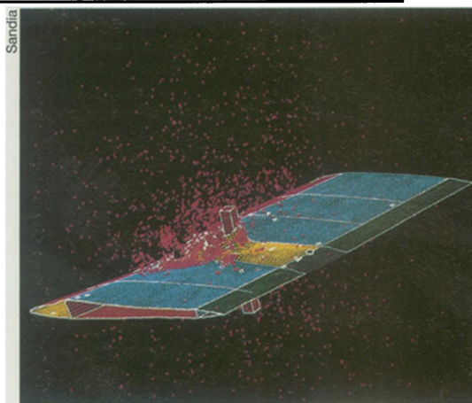
Computer simulation of an airplane wing striking a vertical pole. The ruptured wing sprays fuel, shown by red squares representing the fuel's distribution.
