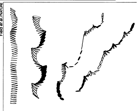
Video images of disks falling through a fluid show that different combinations of disk and fluid properties lead to different types of trajectories (from left to right): steady fall, periodic oscillation, chaotic motion, and tumbling. One side of the disk is white, the other black.
