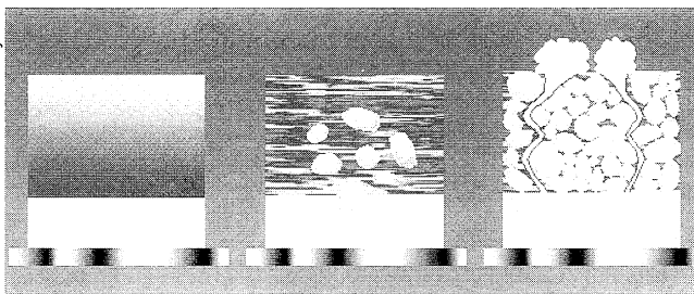
Amorphous solid water (ASW) covers a layer of oily liquid (left). As the temperature increases, the ASW begins to form tiny ice crystals and the oil turns into a gas (center). Once continuous channels through the ASW have formed, gas molecules can escape (right).
