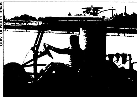
Engineer Mitty C. Plummer of the University of North Texas sits in a prototype vehicle powered by liquid nitrogen, contained in the insulated tank in the rear. The chassis and transmission come from a 1973 Volkswagen.
