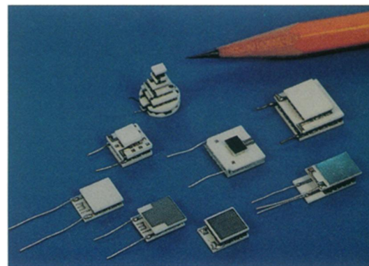
These thermoelectric components, about the size of the end of a pencil, have several cooling stages stacked on top of each other.
