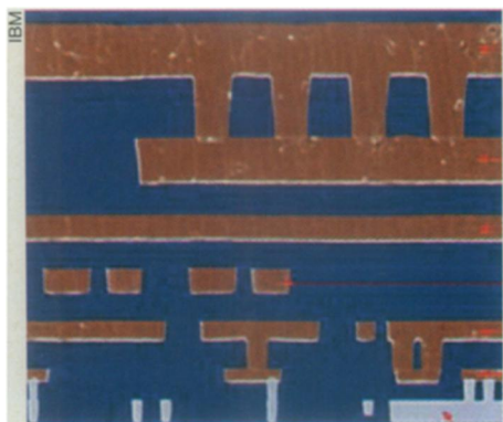
A scanning electron micrograph shows a cross-section of a computer chip made with six layers of copper.
