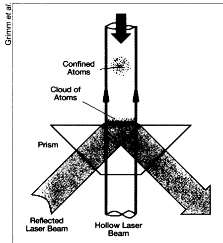
In the gravito-optical surface trap, cesium atoms are initially confined in a magnetic field and slowed down by laser beams. Gravity then pulls the atoms downward. At the surface of a prism, illuminated from below by a laser beam, the atoms interact with the reflected beam's electromagnetic field and rebound, losing some of their energy. Eventually, the atoms collect in a cloud just above the prism. A hollow, vertical laser beam encircling the atoms keeps them from spreading out horizontally.
