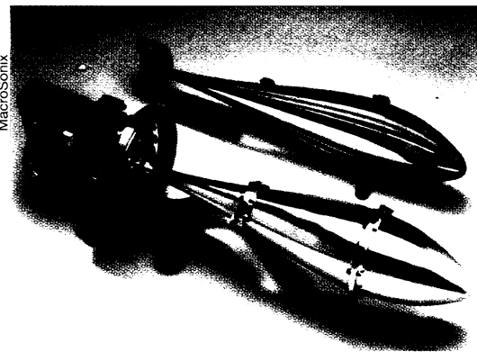
To generate a large-amplitude standing sound wave inside a specially shaped, gas-filled cavity, a motor (front, left) drives the elongated, tapered metal container, about 0.5 meter long, back and forth at a frequency of approximately 600 cycles per second. The cavity itself (shown in cutaway at back) contains no mechanical parts.
